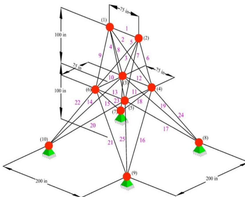
Figure 9. 25-bar truss structure
